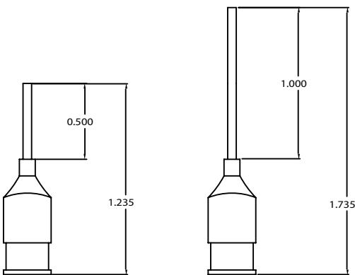
Luer Lock Caps Part Number: PVA-LLCAP-X
